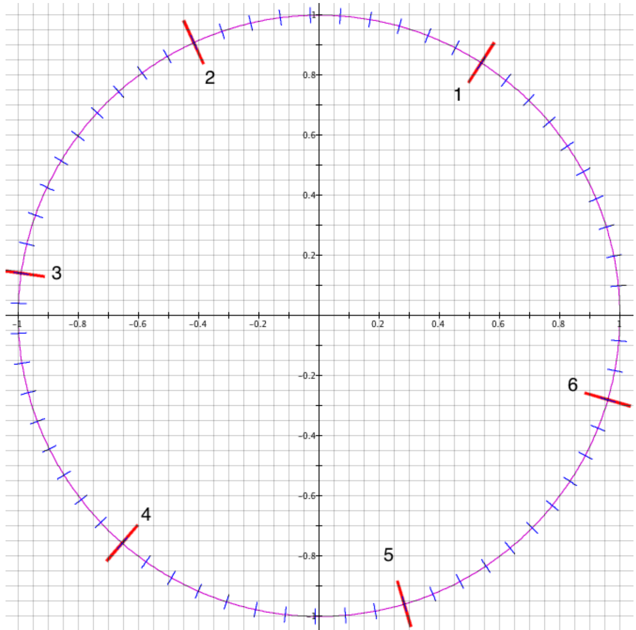
Positive radian ruler (c) 2015 P. Thompson
