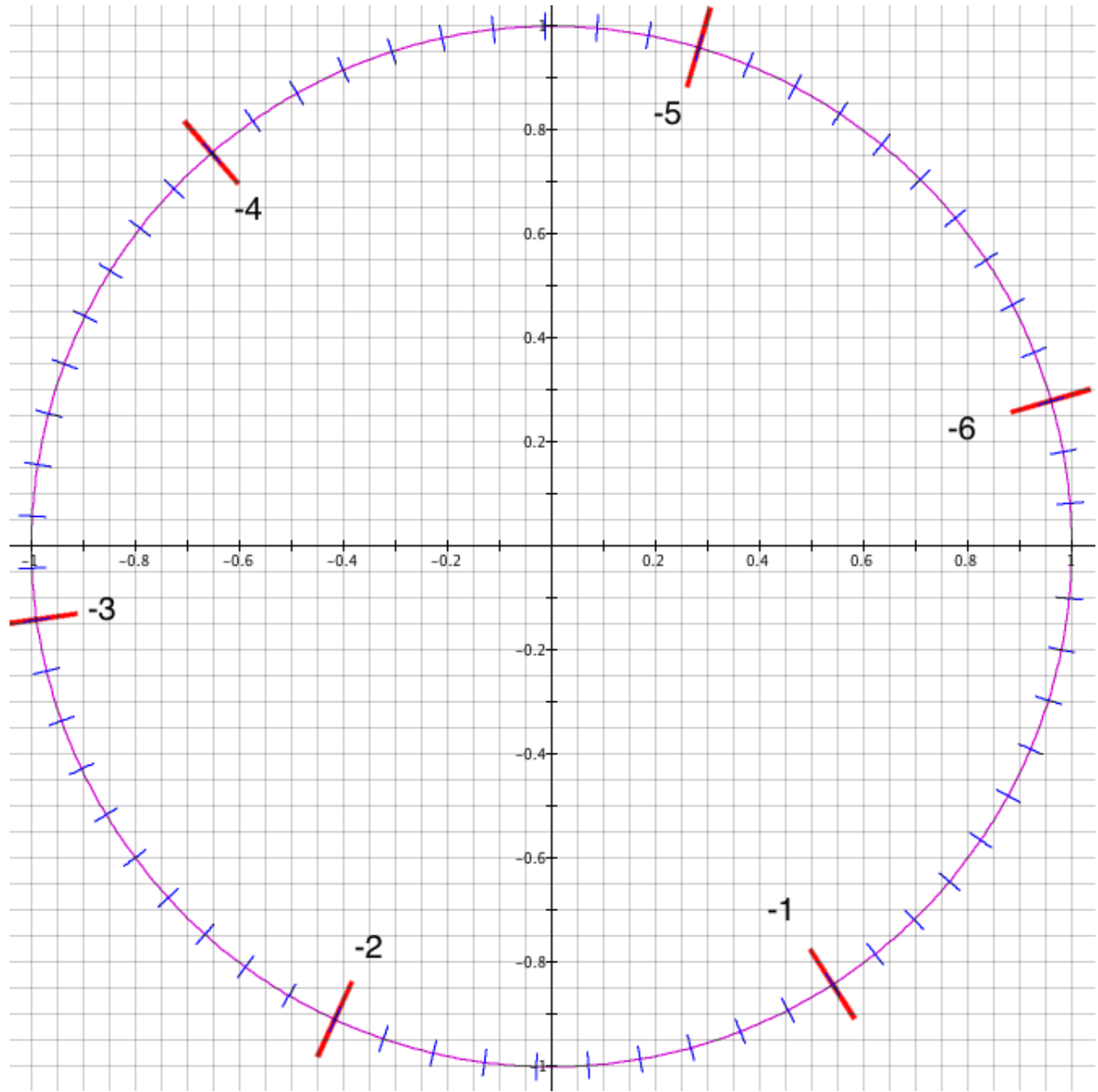
Negative radian ruler (c) 2015 P. Thompson
